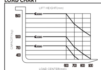
LOAD CHART
